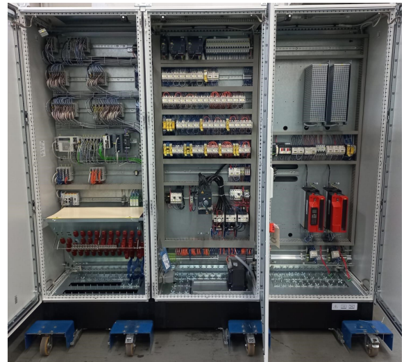
Example of control cabinet with a DataView Full retrofit
